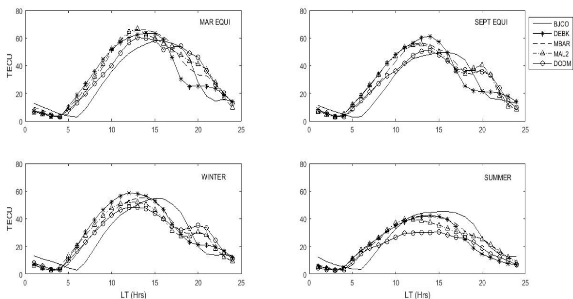
Fig. 4. Seasonal variation of TEC in the year 2013
