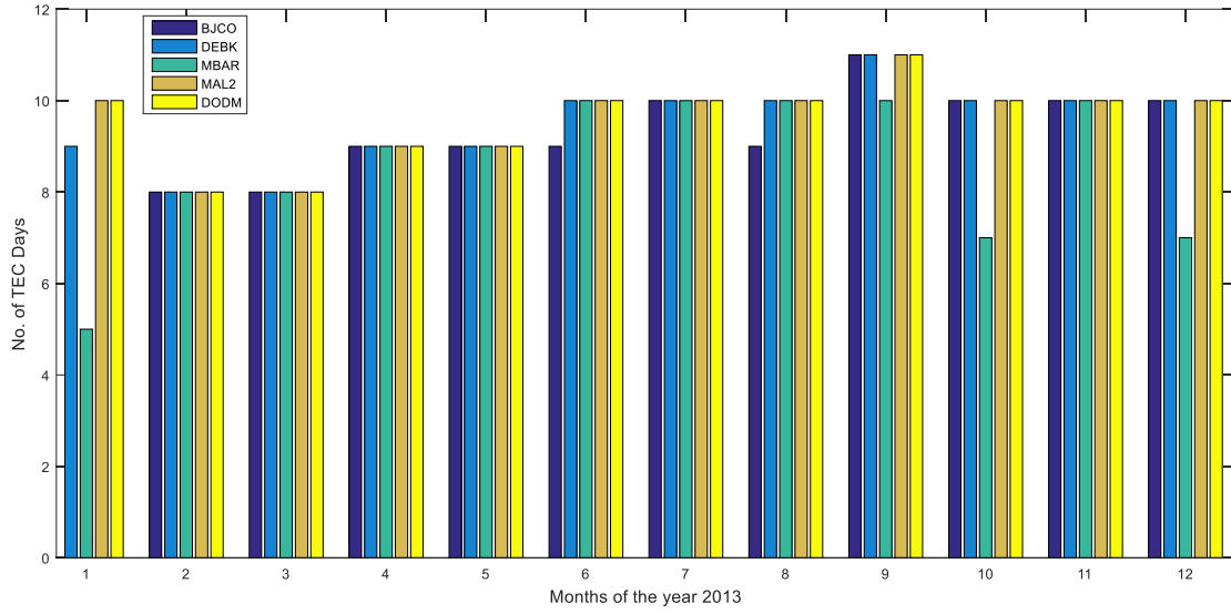
Fig. 1. Histogram depicting the number of available quiet days with A_p \leq 6 used in the study
