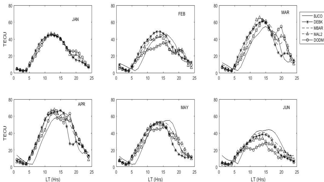
Fig. 3a. Monthly diurnal TEC for January to June during moderate solar activity year 2013
