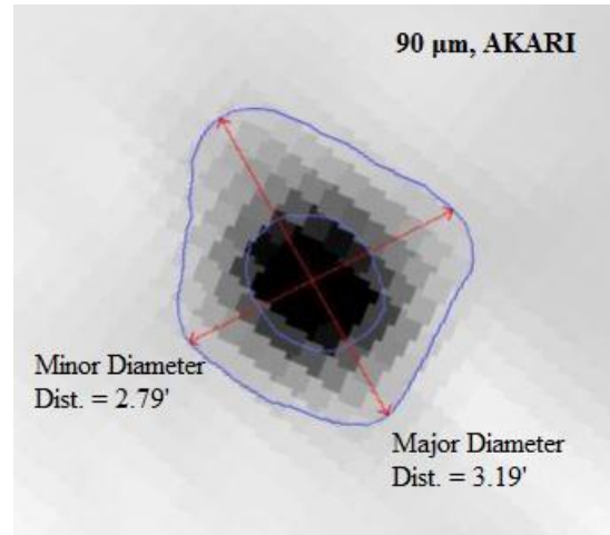
Fig. 5. Major and minor diameter of the nebula structure
