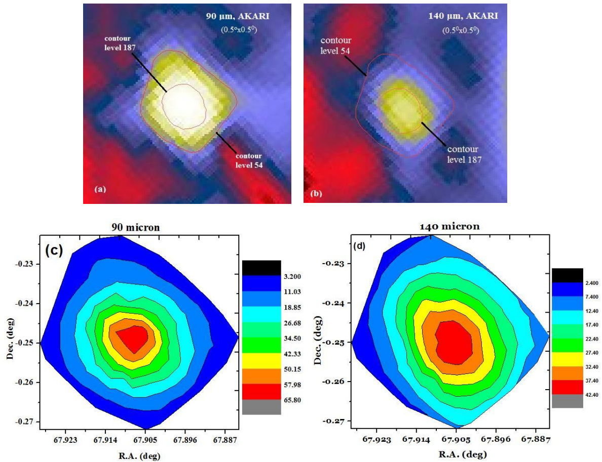
Fig. 1. (a) 0.5°x0.5° FITS image of the structure at 90 \mu m AKARI map. (b) 0.5°x0.5° FITS image of the structure at 140 \mu m AKARI map. (c) Contour map at 90 \mu m flux density. (d) Contour map at 140 \mu m flux density where the PNe is located at R.A. = 67.907°, Dec. = -0.249° (Galactic)
