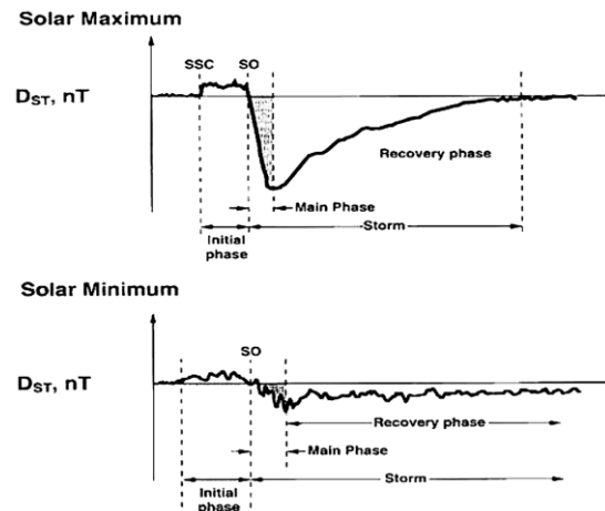
Fig. 4. The behaviour of Dst during solar maximum and minimum
