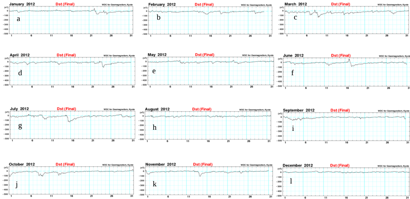
Fig. 12(a – I). Plots of the Dst final for all the months in the year 2012 Source: WDC for Geomagnetism, Kyoto
