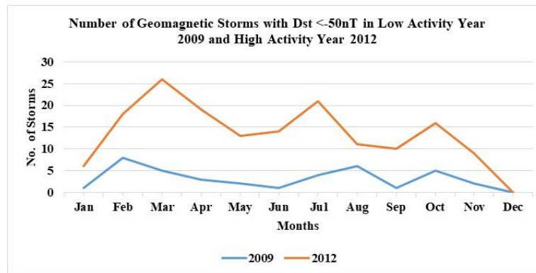
Fig. 13. Plots of SSC in 2009 and 2012 showing the peaks
