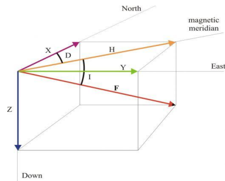
Fig. 10. The elements of earth's magnetic field
