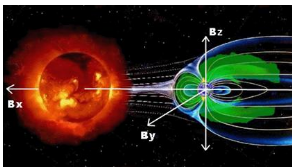
Fig. 1. The connection between the IMF and the earth's magnetosphere
