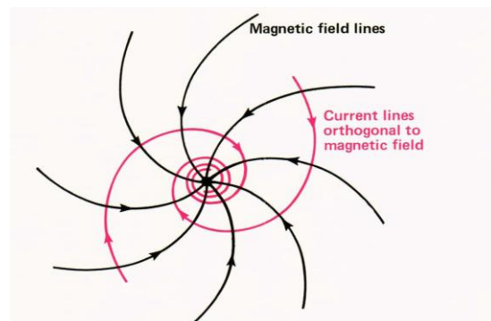
Fig. 2. The Parker Spiral
