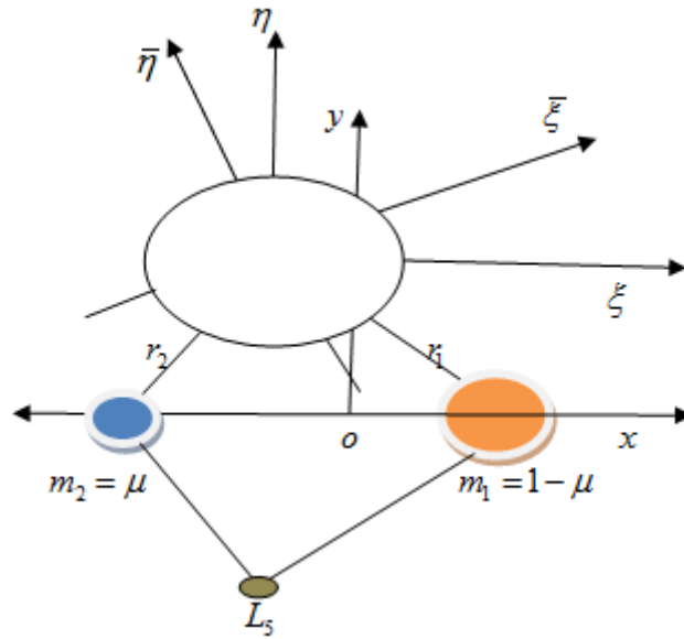
Fig. 1. Orientation of the principal axes for the periodic orbits
