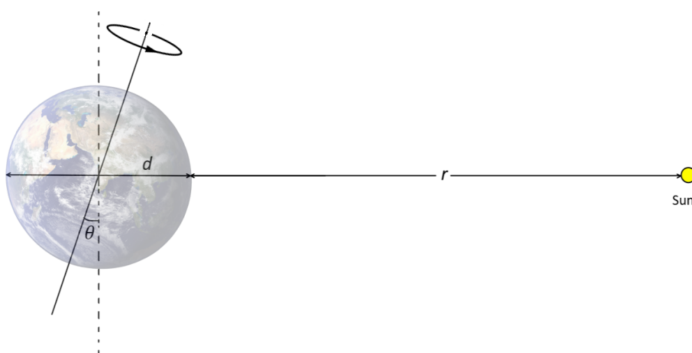
Fig. 1. The side view of a planet representing the quantities of the parent equation (not to scale)
