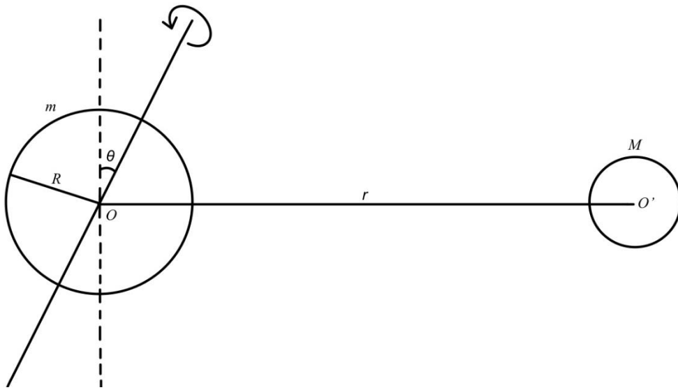
Fig. 2. The planetary system (not to scale)
