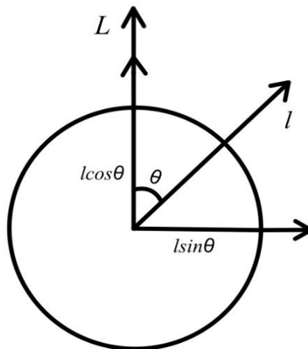
Fig. 3. Angular momenta of a planet
