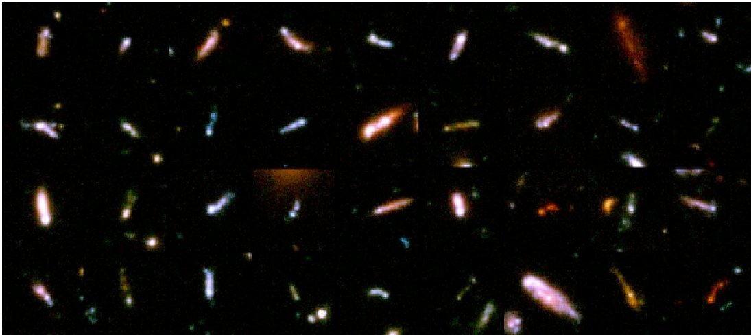
Fig. 10. A gallery of 36 Tadpole galaxies.
