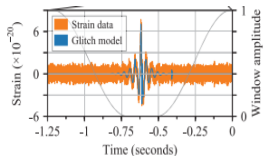
Fig. 10. Noise wave patterns during binary neutron star merger
