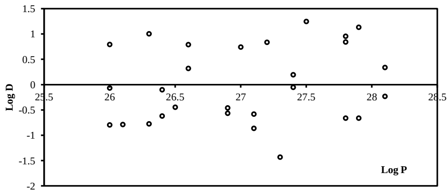
Fig. 4. The scatter plot of source observed linear sizes against observed luminosities for the CSS radio galaxies
