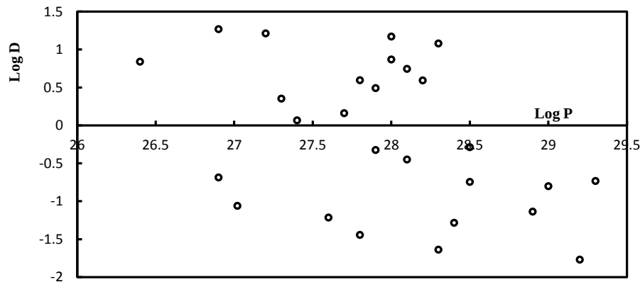
Fig. 2. The scatter plot of source observed linear sizes against observed luminosities for the CSS quasars
