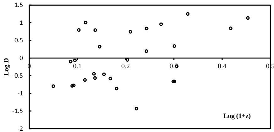
Fig. 3. The scatter plot of source observed linear sizes against observed redshifts for the CSS radio galaxies
