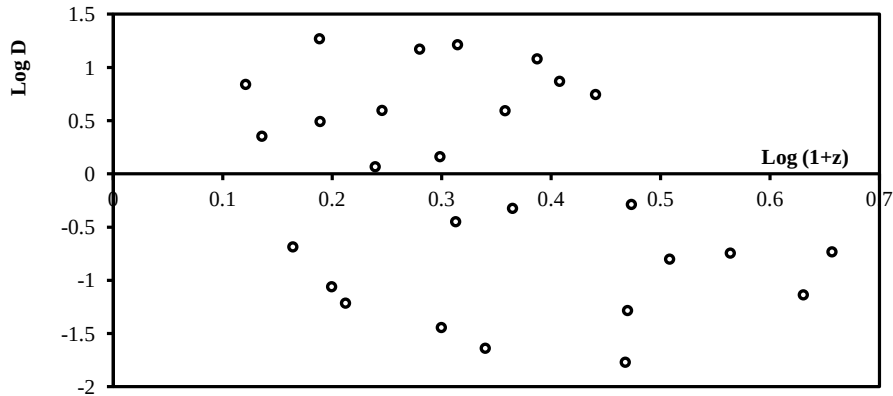
Fig. 1. The scatter plot of linear size against redshift for the CSS quasars
