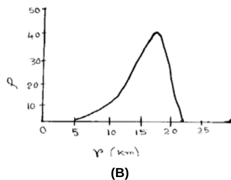
Fig. 1. Schematic diagram showing (A) the structure of a hollow sphere neutron star (not scaled). r_c \rightarrow Center of the hollow neutron star. r_{in} \rightarrow radius of the inner surface boundary and r_{out} \rightarrow radius of the boundary surface of the hollow Neutron Star, respectively. Dark black shaded area marked "maximum density" indicates mass density and pressure are maximum whose location is somewhere between inner and outer surface boundaries of the hollow neutron star; (B) density ' \rho ' – radius ' r ' curve as per Ni's solution which clearly indicates mass density and pressure with initial value zero at the inner surface boundary, then reach maximum value somewhere and again reach to zero at the boundary surface of the hollow neutron star as per Ni's solution
