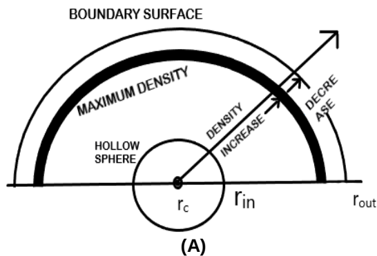
Fig. 1. Schematic diagram showing (A) the structure of a hollow sphere neutron star (not scaled). r_c \rightarrow Center of the hollow neutron star. r_{in} \rightarrow radius of the inner surface boundary and r_{out} \rightarrow radius of the boundary surface of the hollow Neutron Star, respectively. Dark black shaded area marked "maximum density" indicates mass density and pressure are maximum whose location is somewhere between inner and outer surface boundaries of the hollow neutron star; (B) density ' \rho ' – radius ' r ' curve as per Ni's solution which clearly indicates mass density and pressure with initial value zero at the inner surface boundary, then reach maximum value somewhere and again reach to zero at the boundary surface of the hollow neutron star as per Ni's solution
